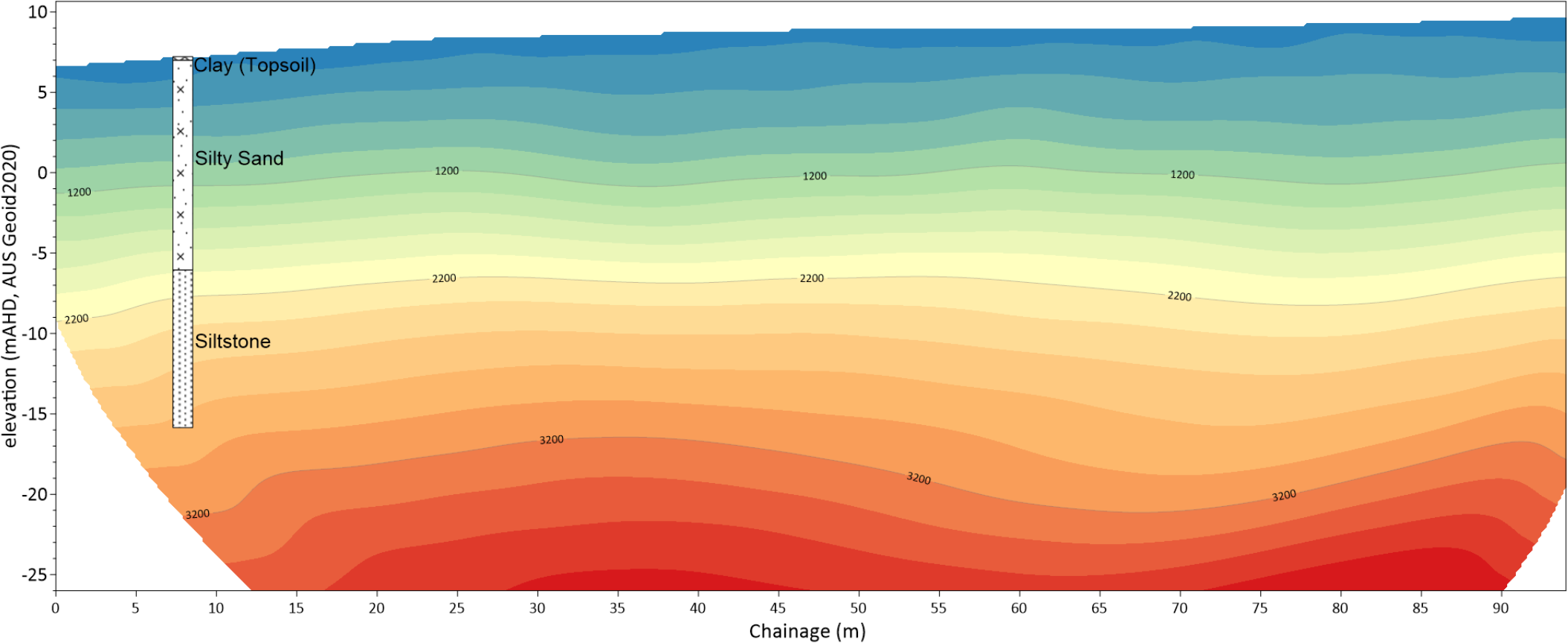
Seismic Line SR AU-GP 143-2
